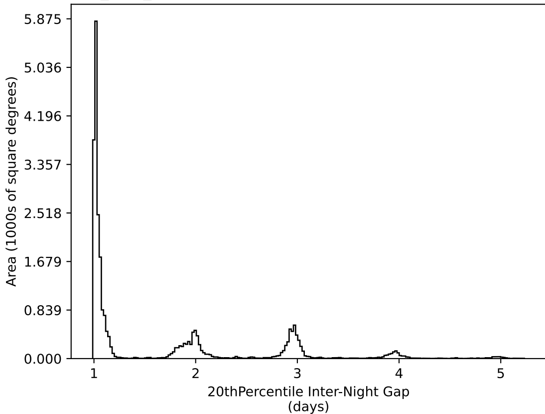
baseline_v2.0_10yrs All sky all bands: 20thPercentile Inter-Night Gap
