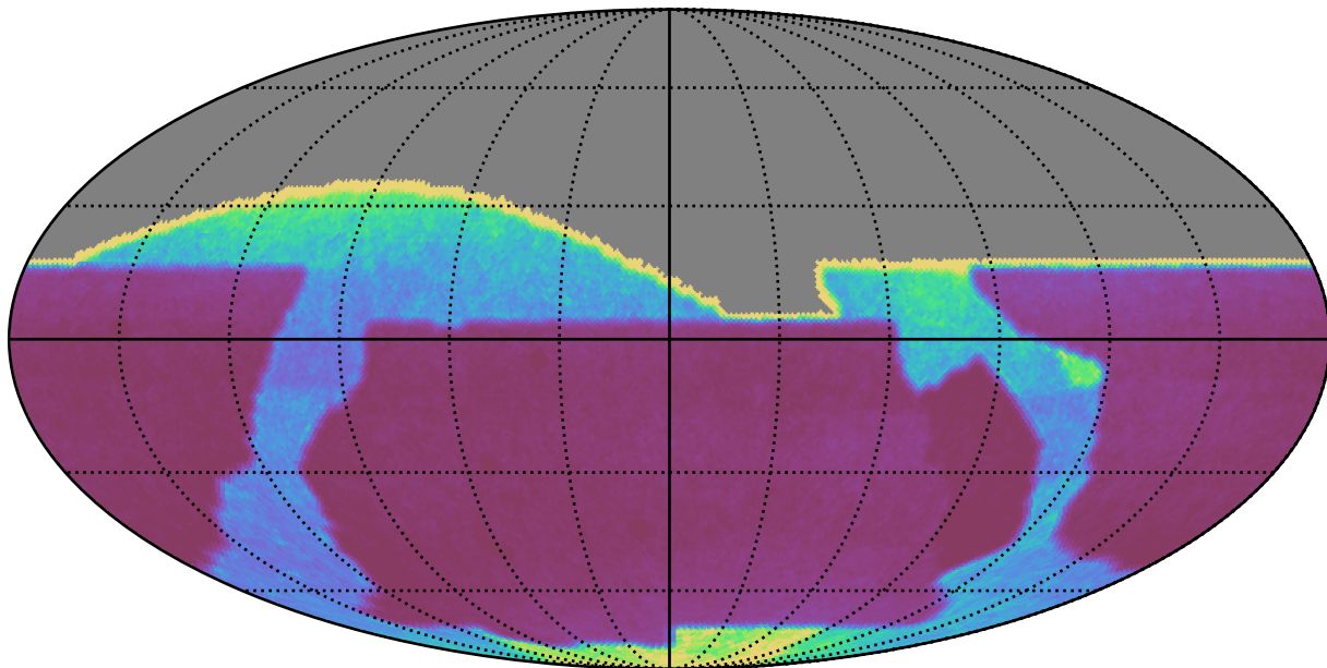
baseline_v2.0_10yrs : properMotion
