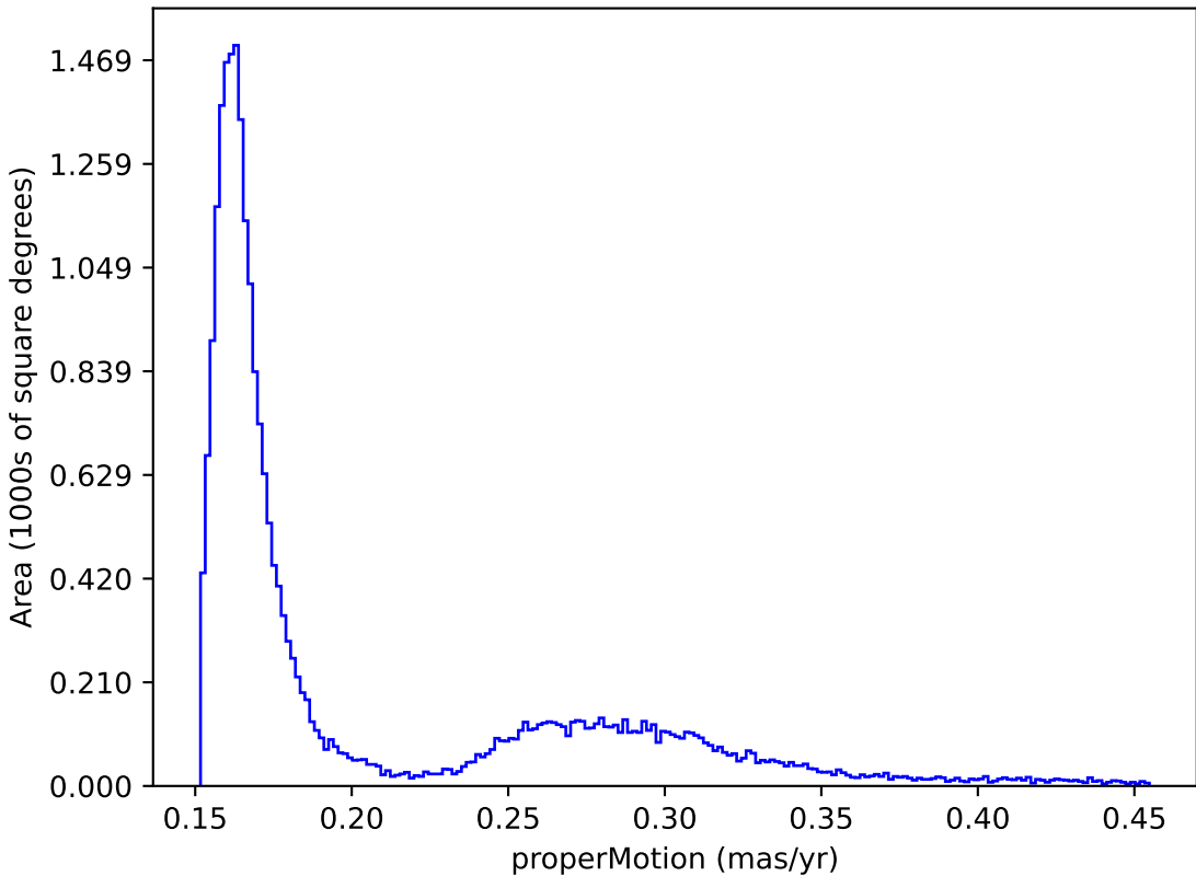
baseline_v2.0_10yrs : properMotion
