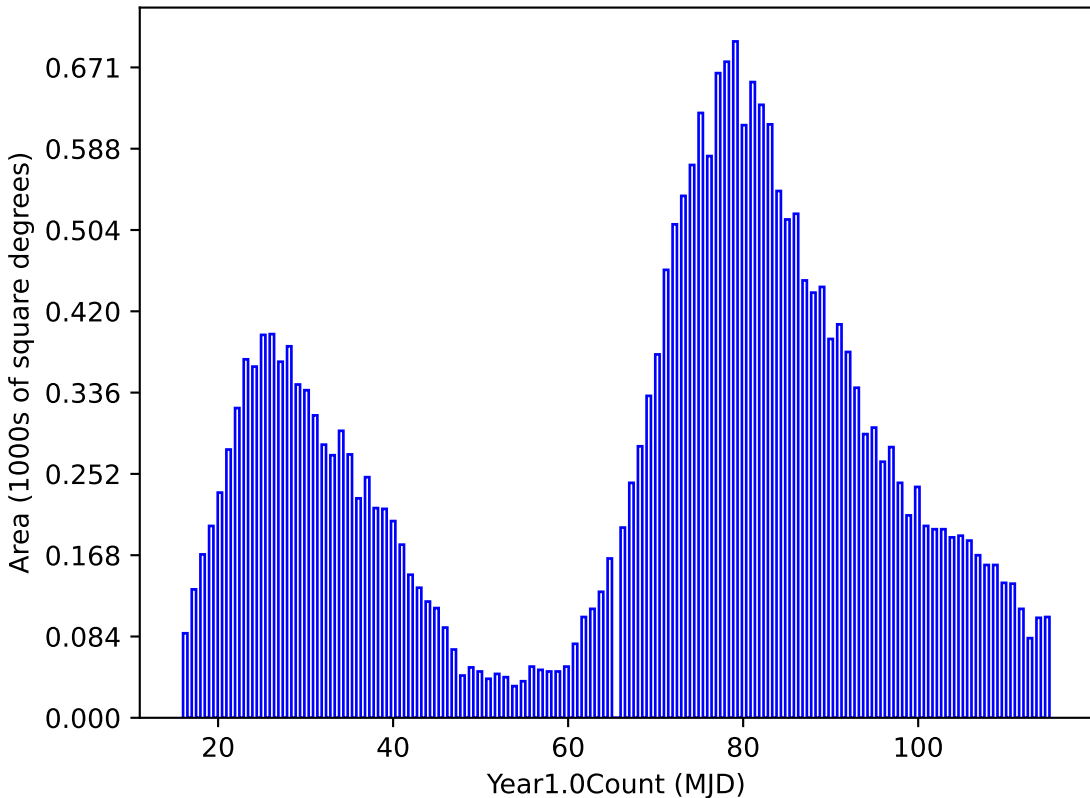
baseline_v2.0_10yrs night < 365.25: Year1.0Count
