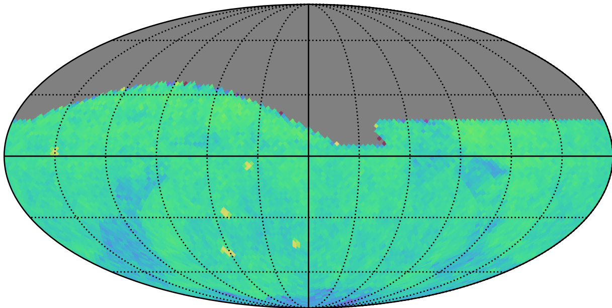
baseline_v2.0_10yrs (g or r or i): PairFraction
