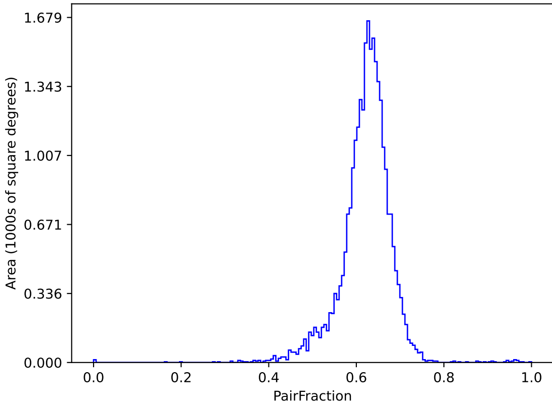
baseline_v2.0_10yrs (g or r or i): PairFraction
