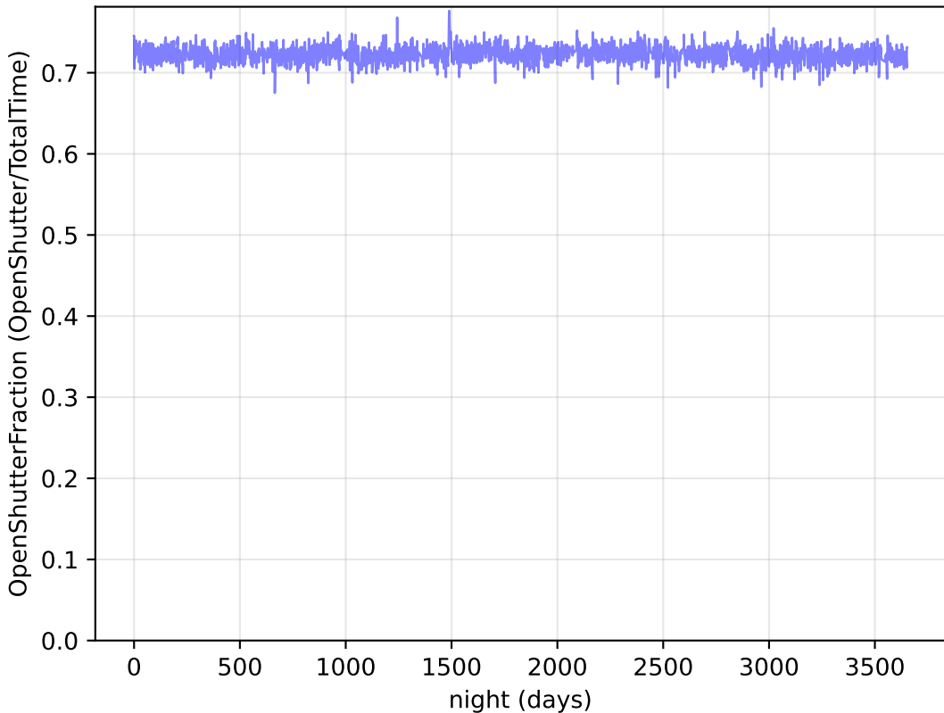
baseline_v2.0_10yrs : OpenShutterFraction
