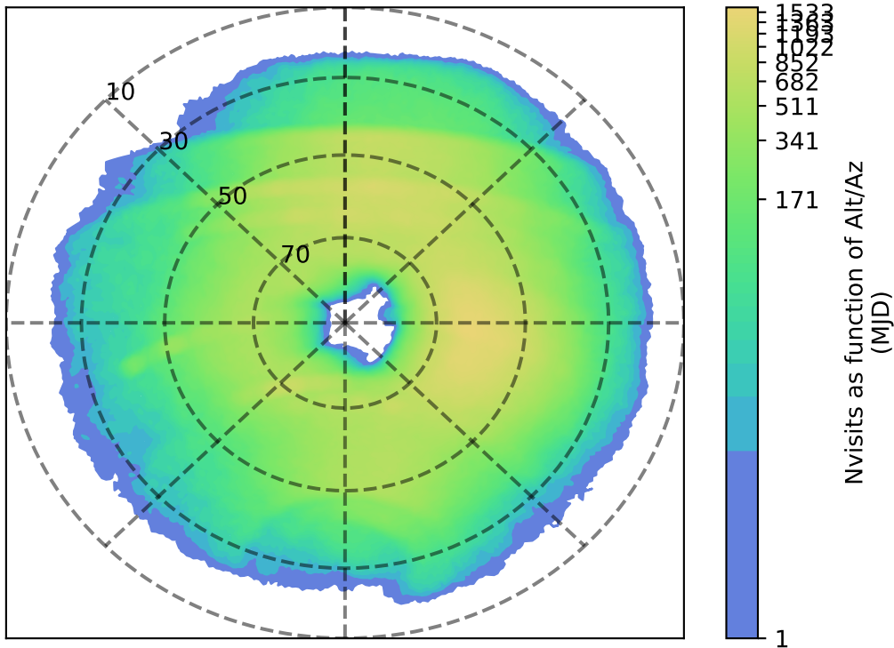
baseline_v2.0_10yrs z: Nvisits as function of Alt/Az
