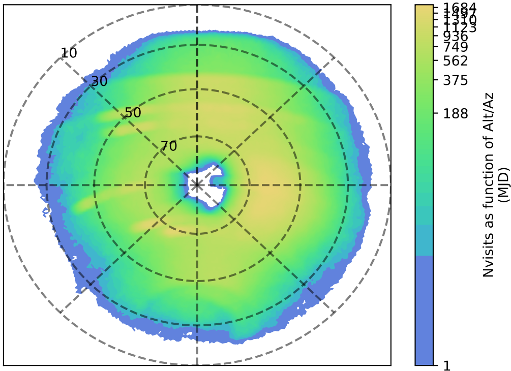
baseline_v2.0_10yrs i: Nvisits as function of Alt/Az
