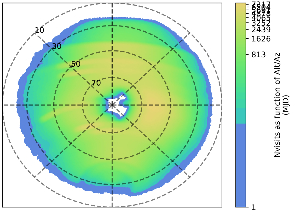
baseline_v2.0_10yrs : Nvisits as function of Alt/Az
