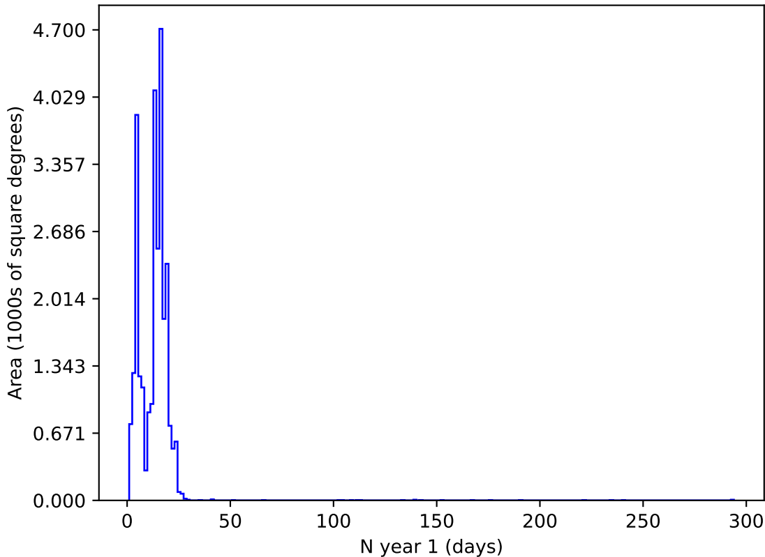
baseline_v2.0_10yrs z and night < 365: N year 1
