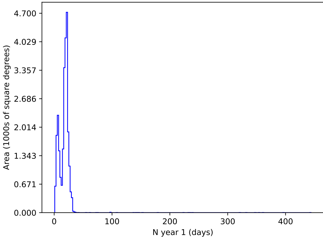
baseline_v2.0_10yrs y and night < 365: N year 1
