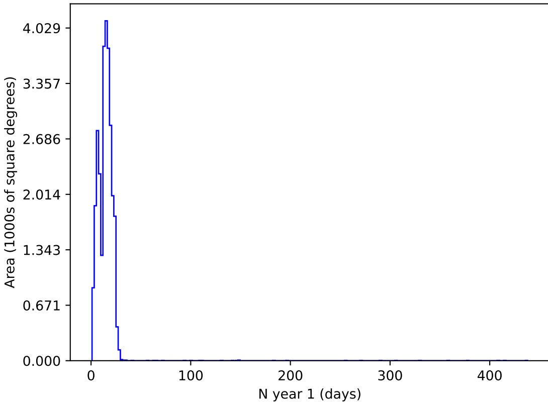
baseline_v2.0_10yrs r and night < 365: N year 1
