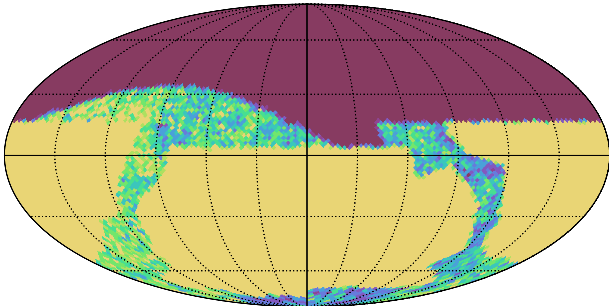
baseline_v2.0_10yrs i and night < 365: N year 1
