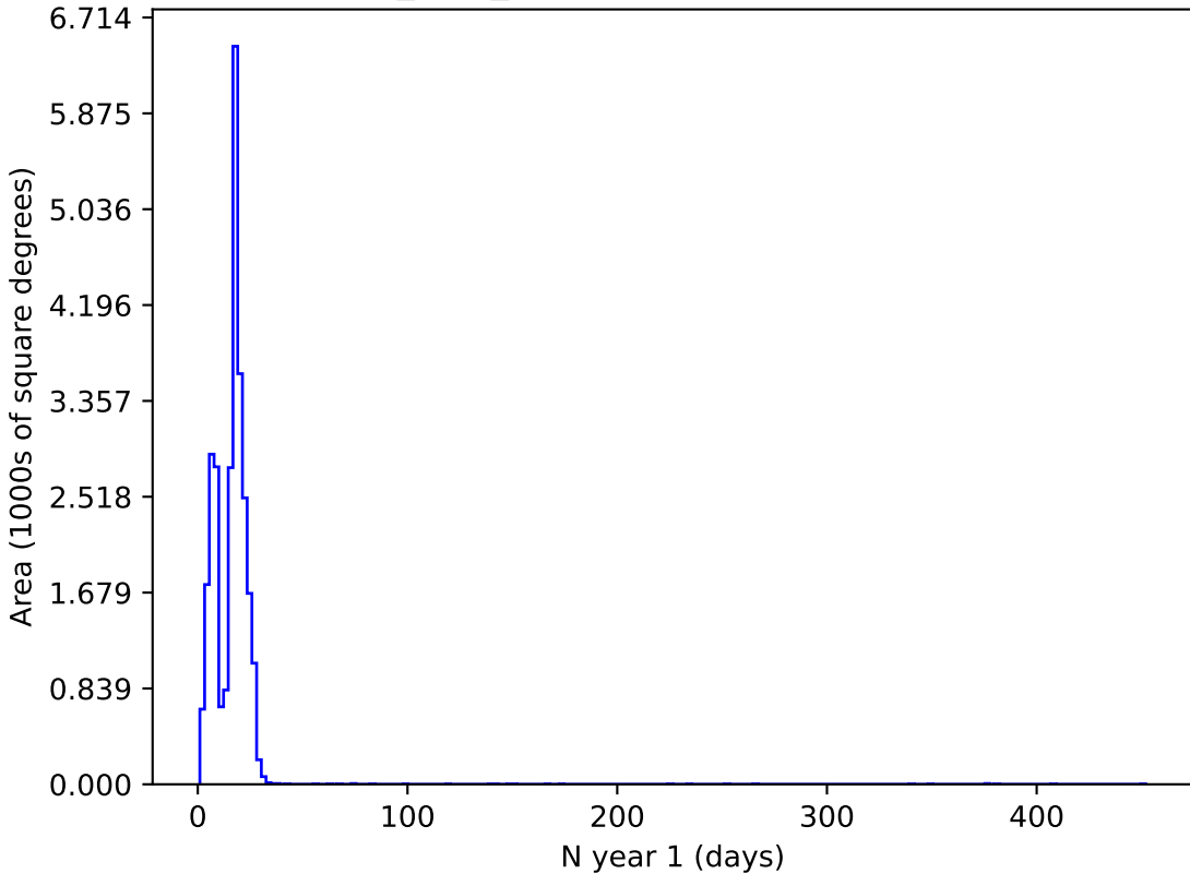
baseline_v2.0_10yrs i and night < 365: N year 1
