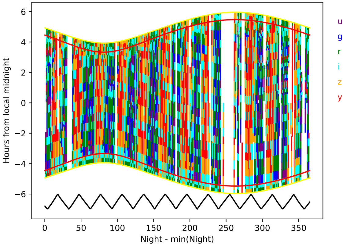
baseline_v2.0_10yrs year 9-10: Hourglass
