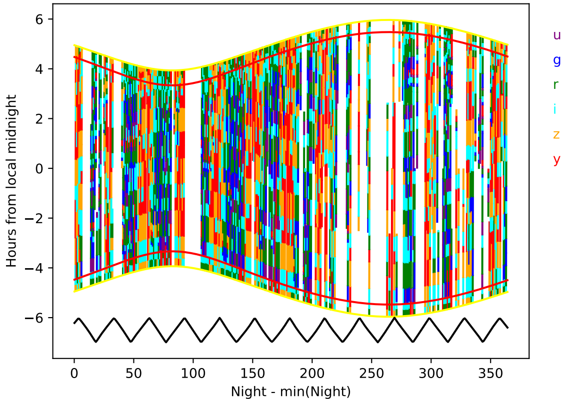
baseline_v2.0_10yrs year 5-6: Hourglass
