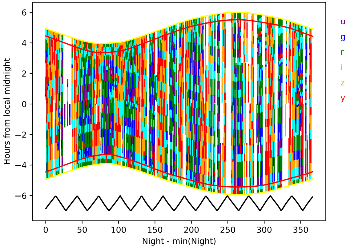
baseline_v2.0_10yrs year 4-5: Hourglass
