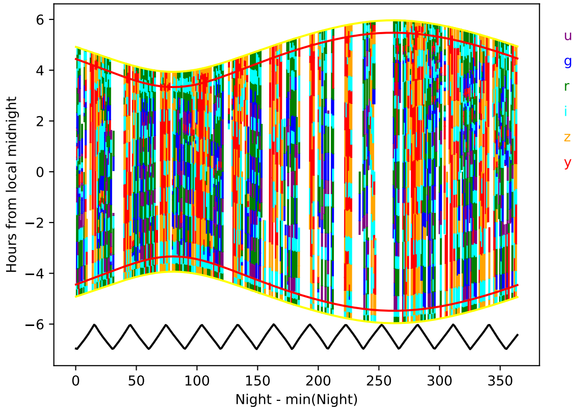
baseline_v2.0_10yrs year 1-2: Hourglass
