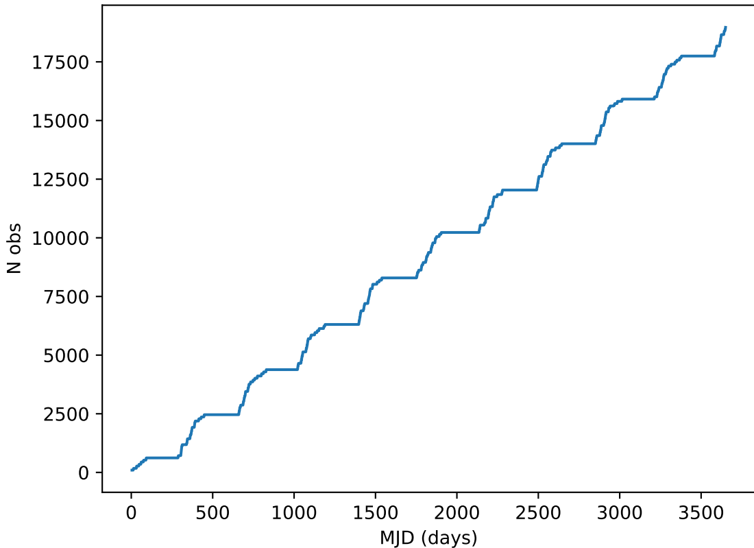
baseline_v2.0_10yrs note like DD:XMM_LSS%: Cumulative
