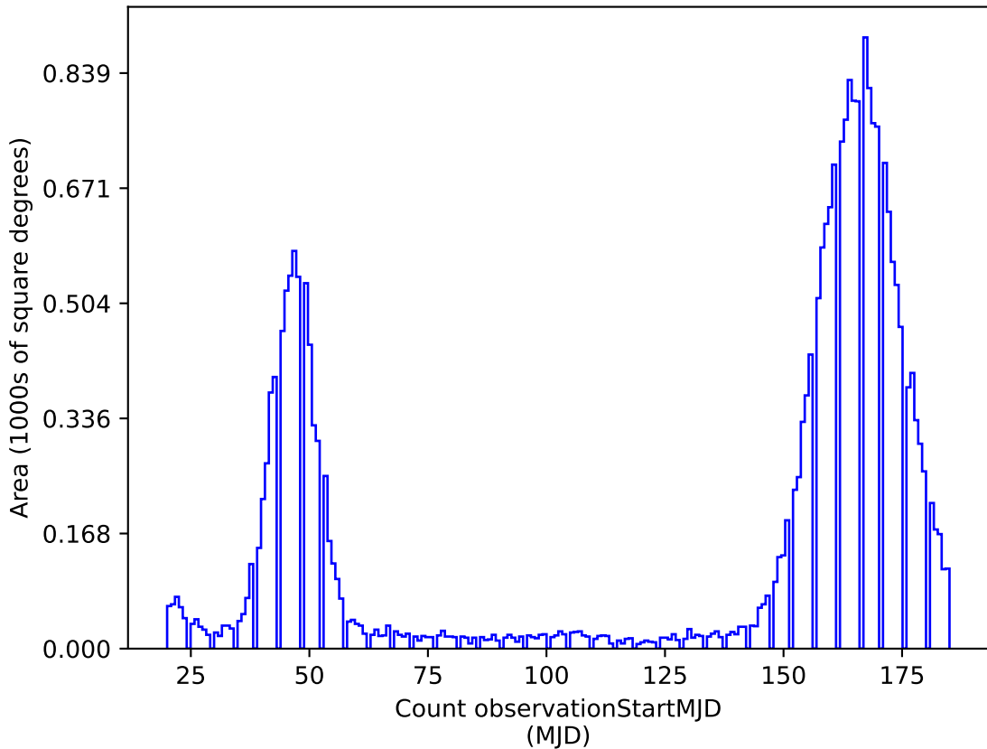
baseline_v2.0_10yrs z: Count observationStartMJD
