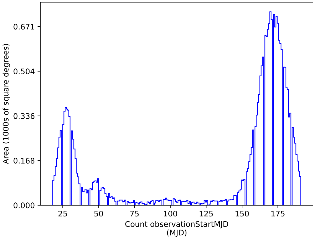
baseline_v2.0_10yrs y: Count observationStartMJD
