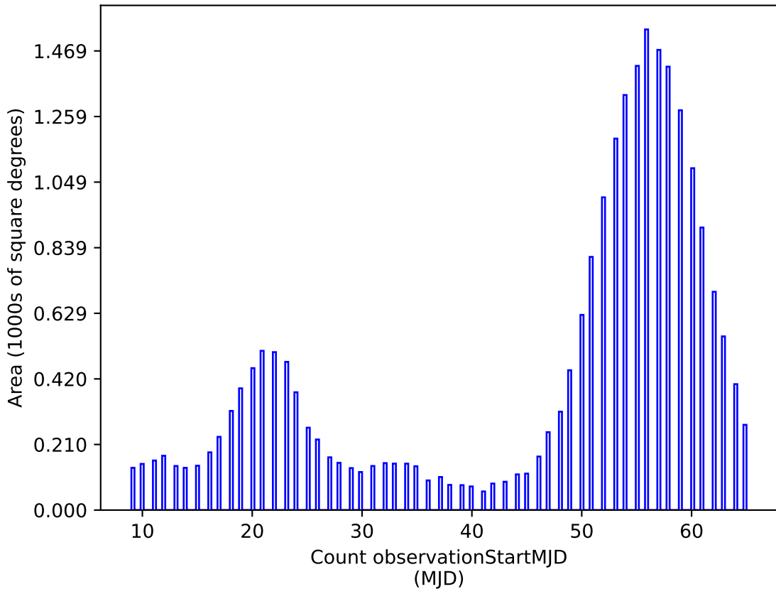
baseline_v2.0_10yrs u: Count observationStartMJD
