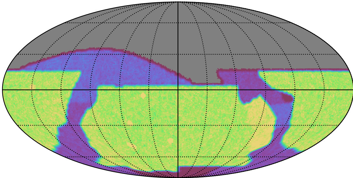
baseline_v2.0_10yrs i: Count observationStartMJD
