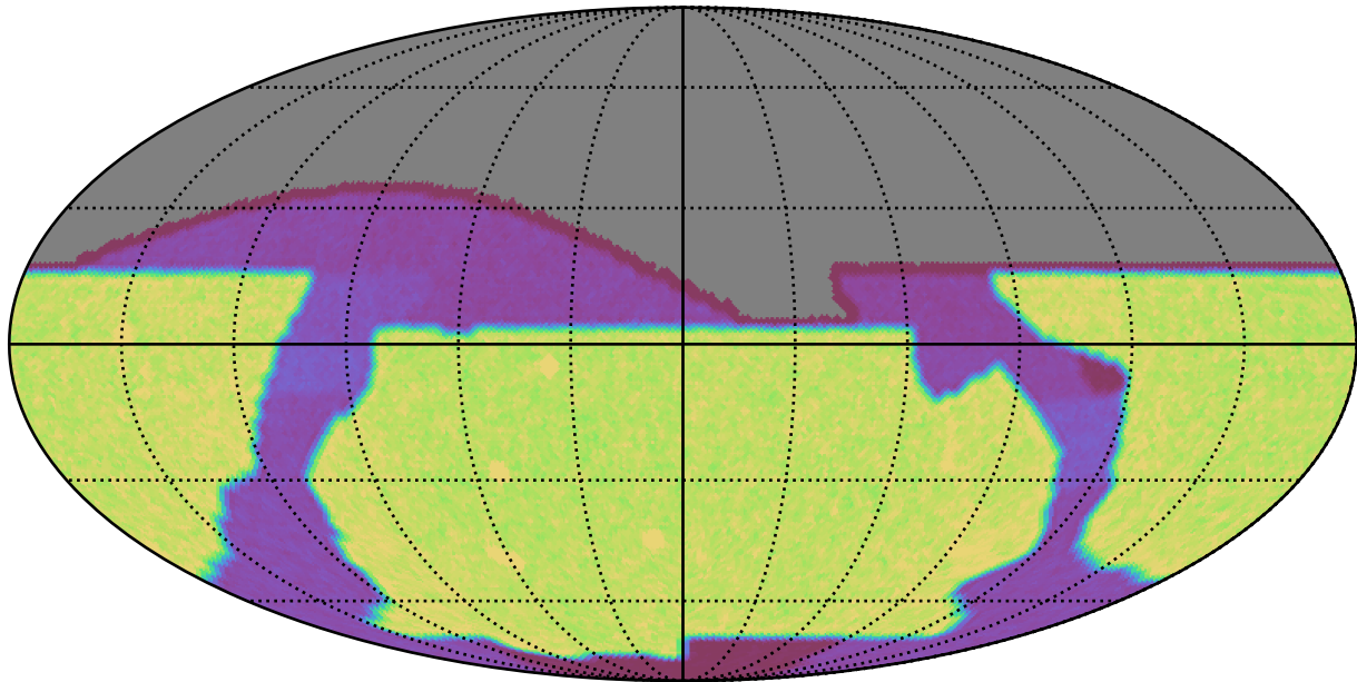
baseline_v2.0_10yrs : Count observationStartMJD
