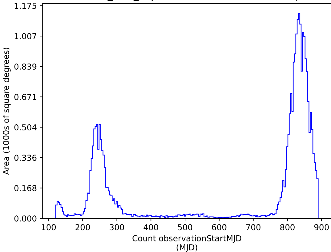
baseline_v2.0_10yrs : Count observationStartMJD
