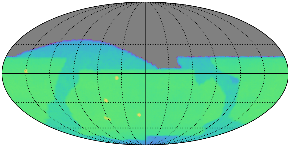
baseline_v2.0_10yrs z: CoaddM5
