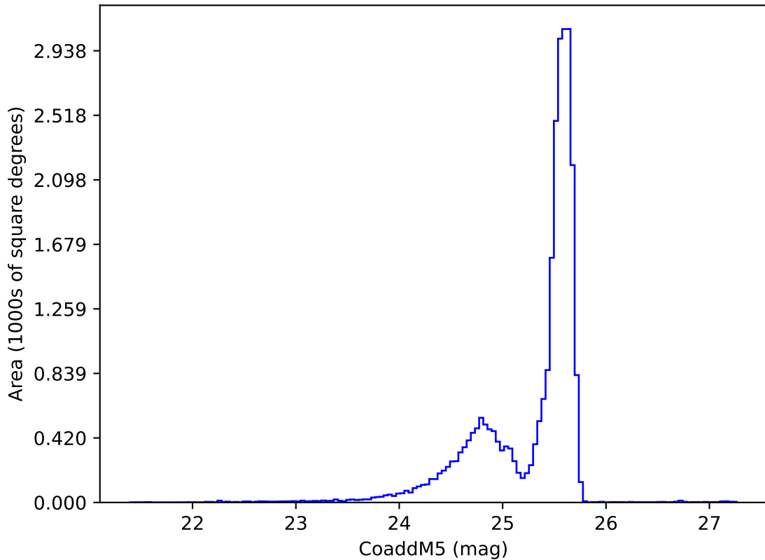
baseline_v2.0_10yrs z: CoaddM5
