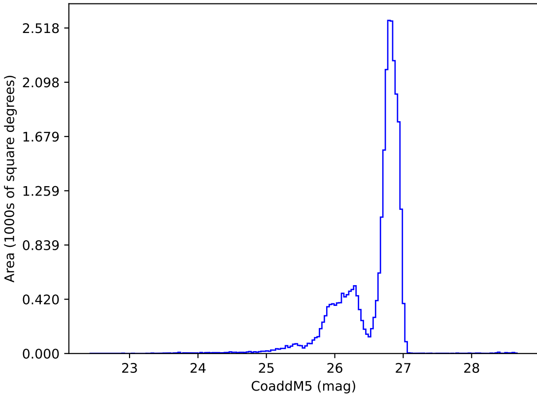
baseline_v2.0_10yrs r: CoaddM5
