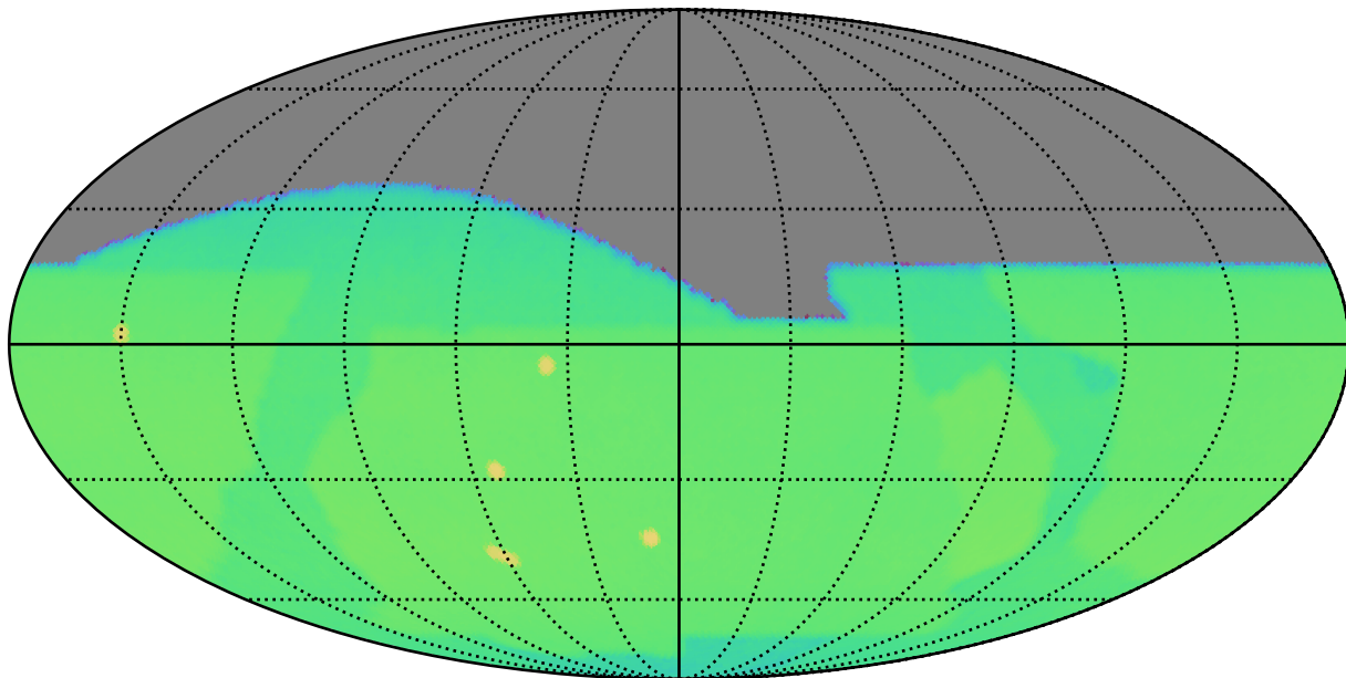
baseline_v2.0_10yrs : CoaddM5
