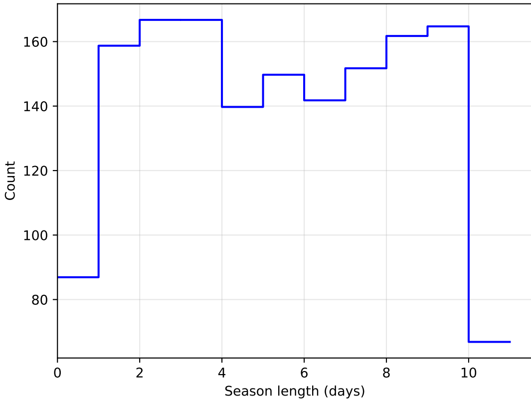
baseline_v2.0_10yrs DD:XMM_LSS all bands: SeasonLength
