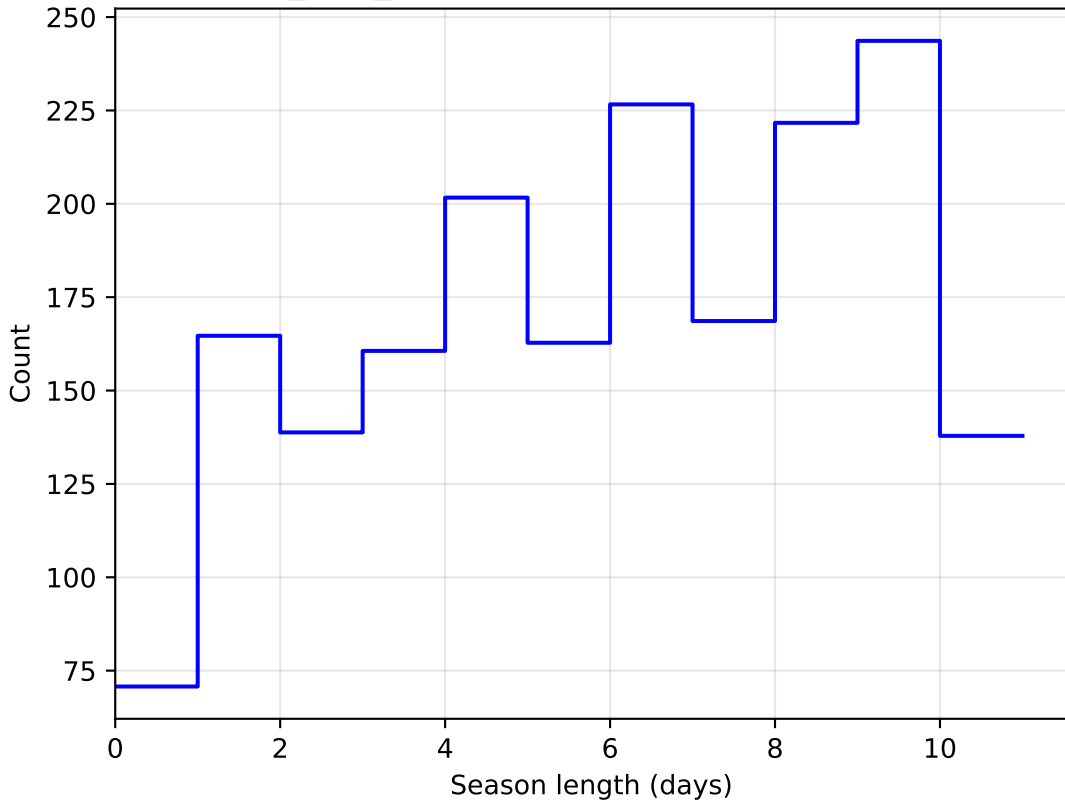
baseline_v2.0_10yrs DD:WFD all bands: SeasonLength
