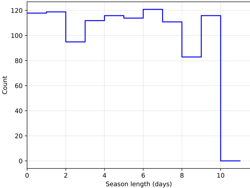
baseline_v2.0_10yrs DD:EDFS all bands: SeasonLength
