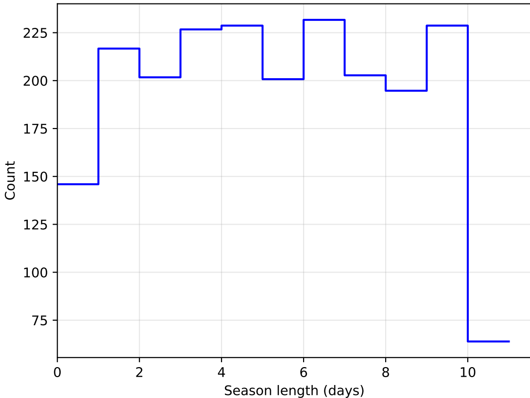
baseline_v2.0_10yrs DD:ECDFS all bands: SeasonLength
