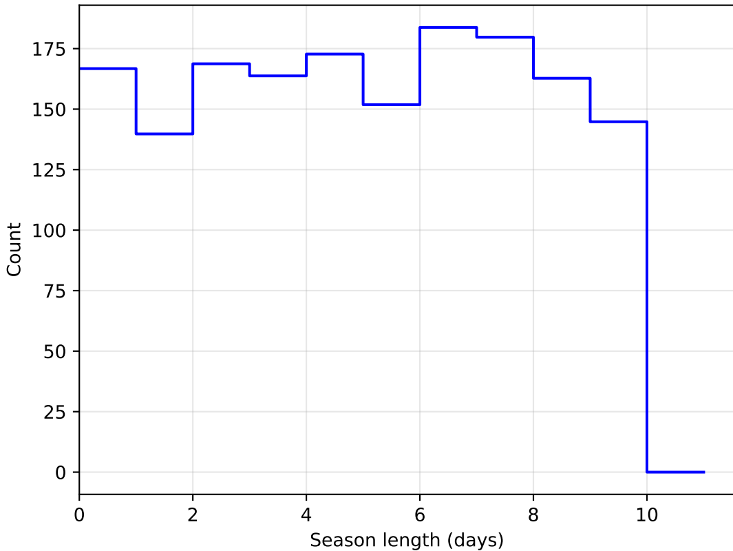
baseline_v2.0_10yrs DD: COSMOS all bands: SeasonLength
