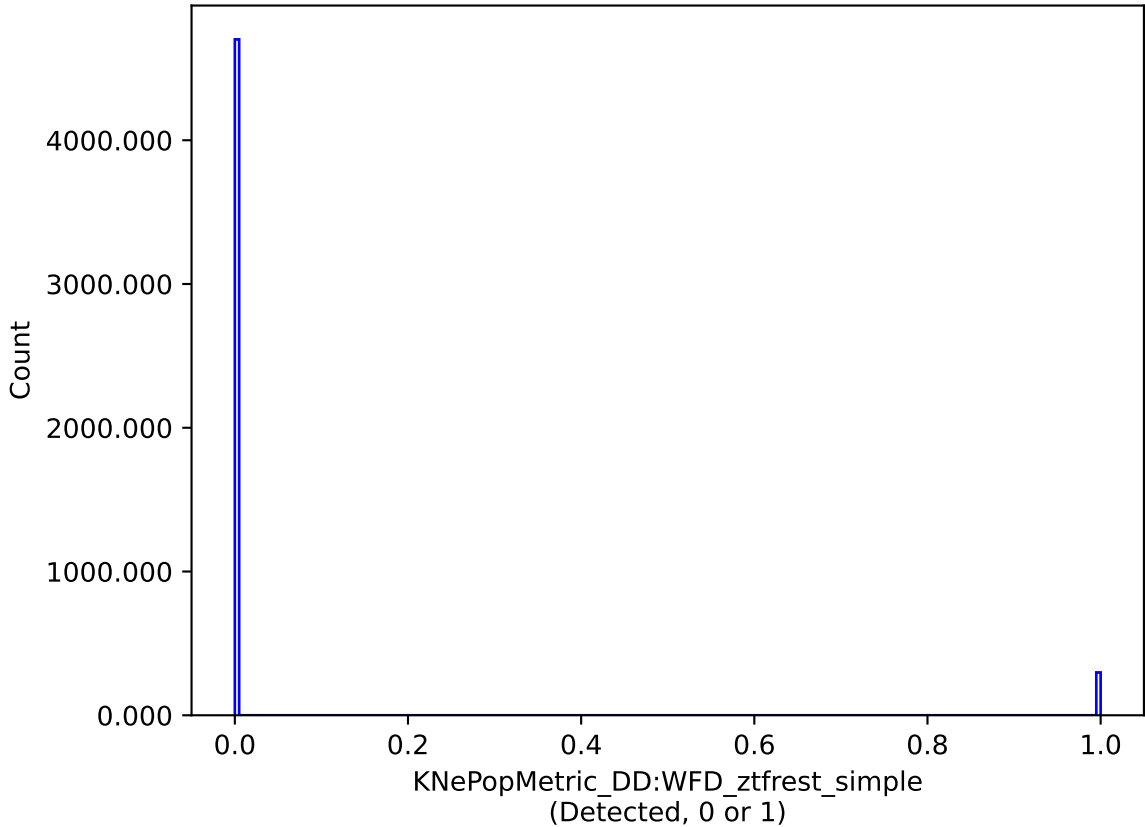
baseline_v2.0_10yrs DD:WFD: KNePopMetric_DD:WFD_ztfrest_simple
