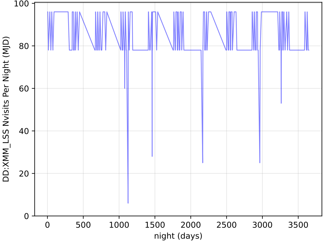
baseline_v2.0_10yrs all bands: DD:XMM_LSS Nvisits Per Night
