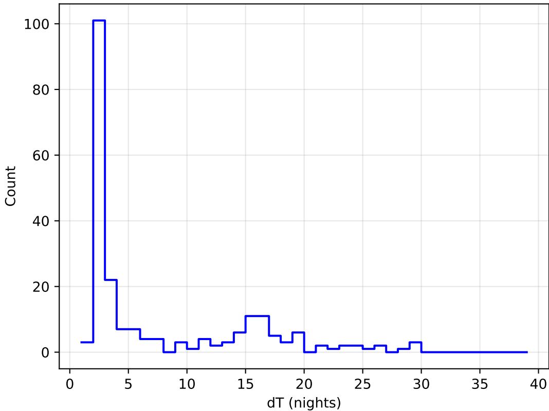
baseline_v2.0_10yrs all bands: DD:XMM_LSS Delta Nights Histogram
