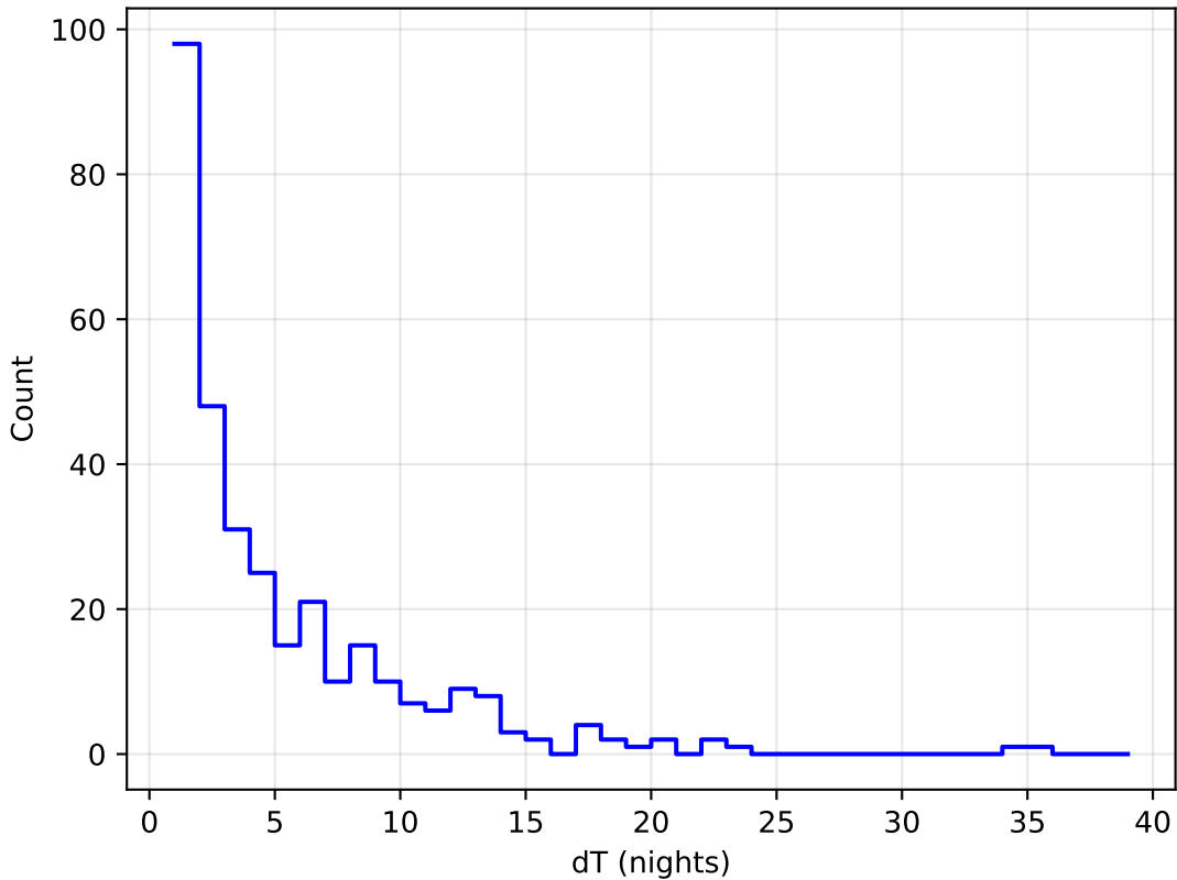
baseline_v2.0_10yrs all bands: DD:WFD Delta Nights Histogram
