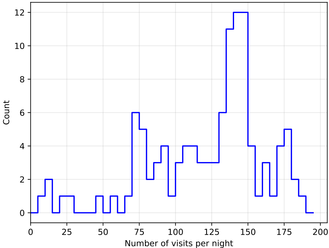
baseline_v2.0_10yrs all bands: DD:EDFS NVisitsPerNight
