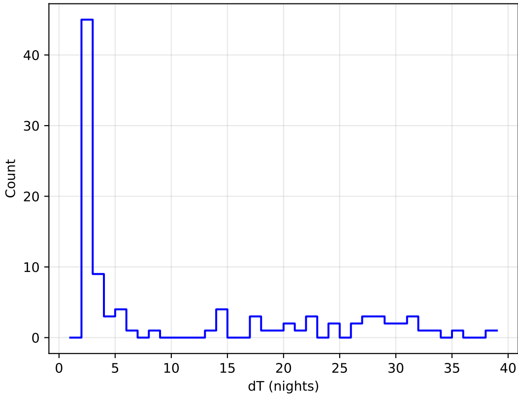
baseline_v2.0_10yrs all bands: DD:EDFS Delta Nights Histogram
