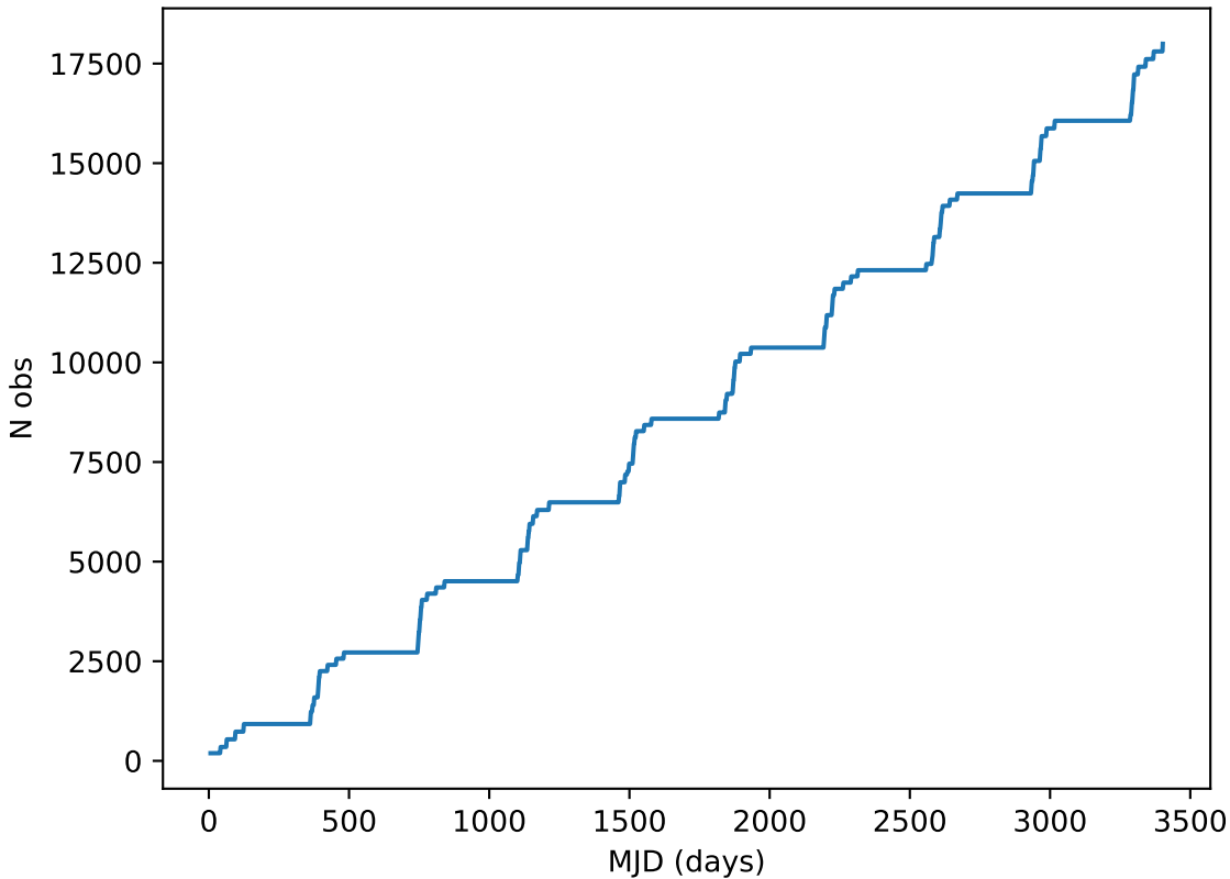
baseline_v2.0_10yrs all bands: DD:EDFS Cumulative NVisits
