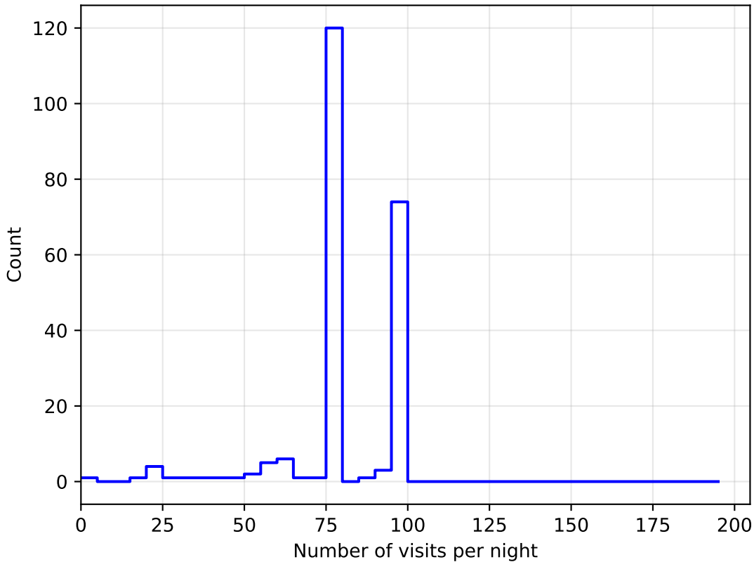
baseline_v2.0_10yrs all bands: DD:ECDFS NVisitsPerNight
