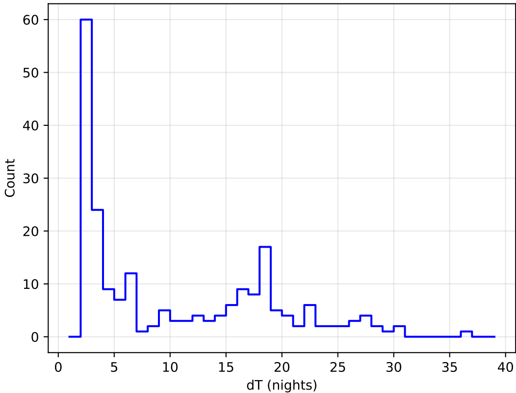
baseline_v2.0_10yrs all bands: DD:ECDFS Delta Nights Histogram
