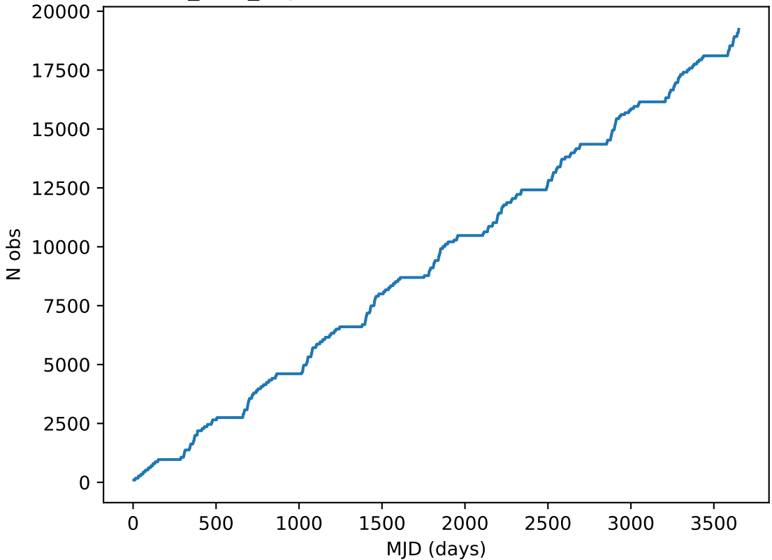
baseline_v2.0_10yrs all bands: DD:ECDFS Cumulative NVisits
