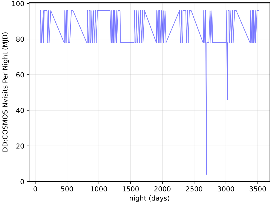
baseline_v2.0_10yrs all bands: DD:COSMOS Nvisits Per Night
