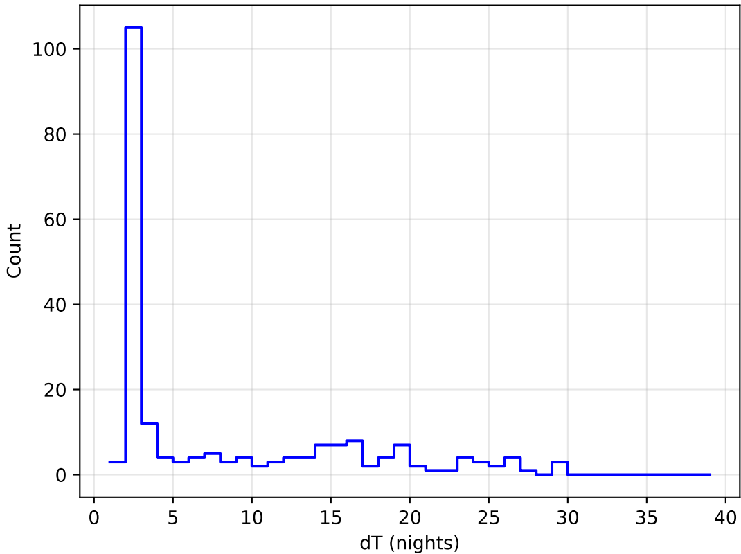
baseline_v2.0_10yrs all bands: DD: COSMOS Delta Nights Histogram
