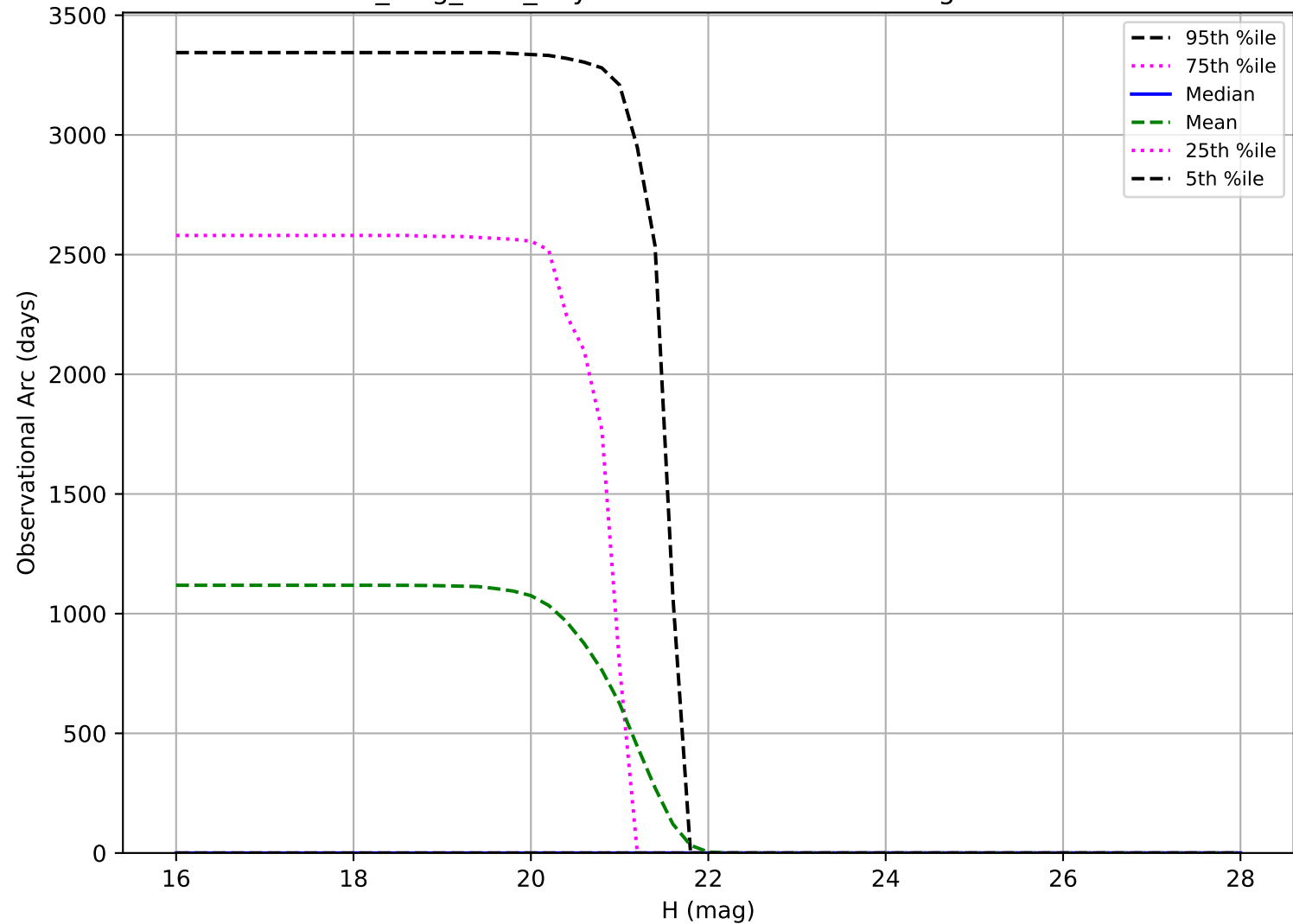
all_long_v3.4_10yrs: Observational Arc Length Vatira
