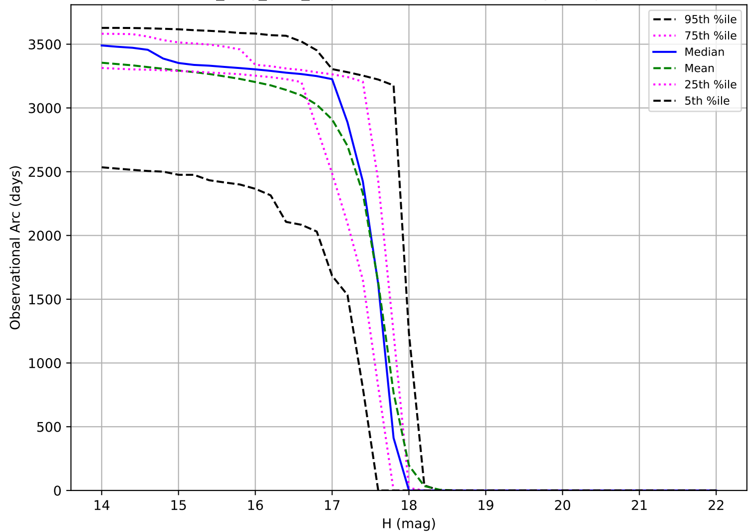
all_long_v3.4_10yrs: Observational Arc Length Trojan
