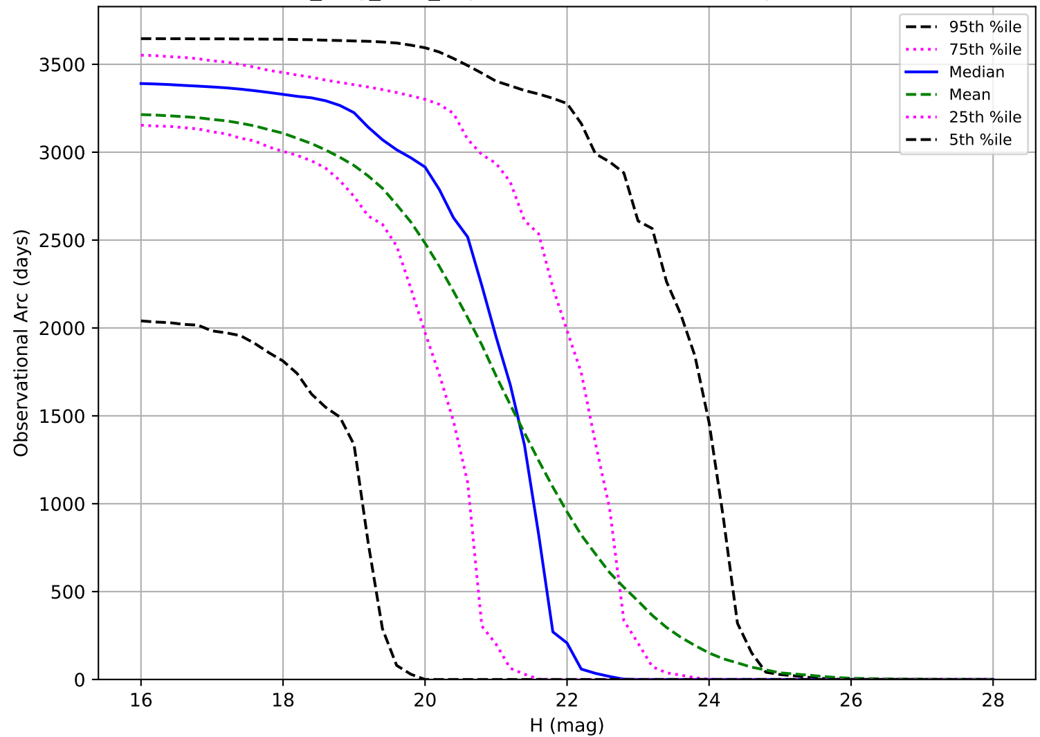
all_long_v3.4_10yrs: Observational Arc Length PHA
